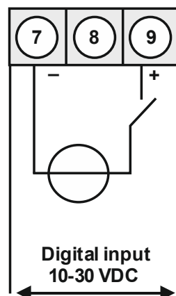
M2 with digital input and external voltage supply source
