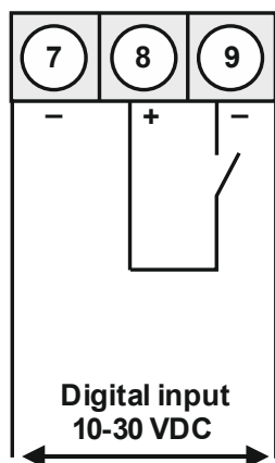
M2 with digital input in combination with 24 VDC sensor supply
